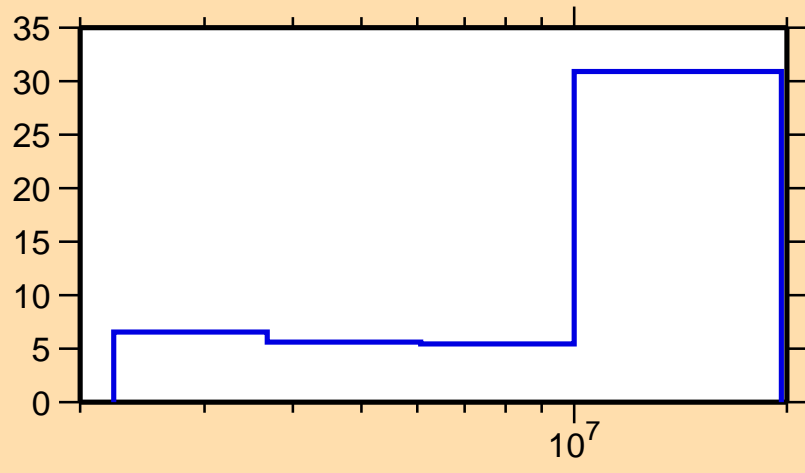
\Delta\sigma/\sigma vs. E for ^{120}\text{Te}(n,n\text{cont.})
