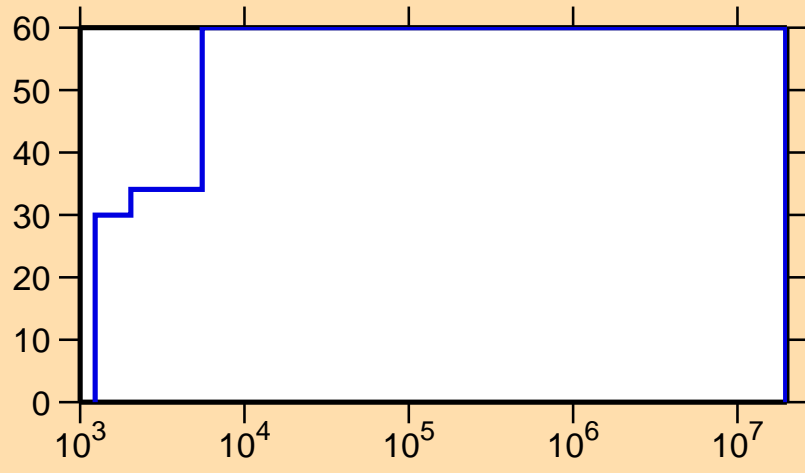
\Delta\sigma/\sigma vs. E for ^{121}\text{Te}(n,\gamma)
