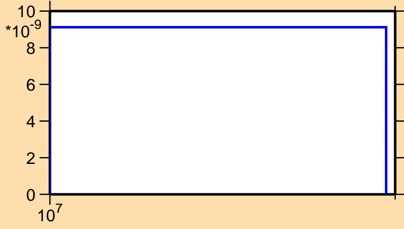
\sigma vs. E for ^{121}\text{Te}(n,\text{He3})
