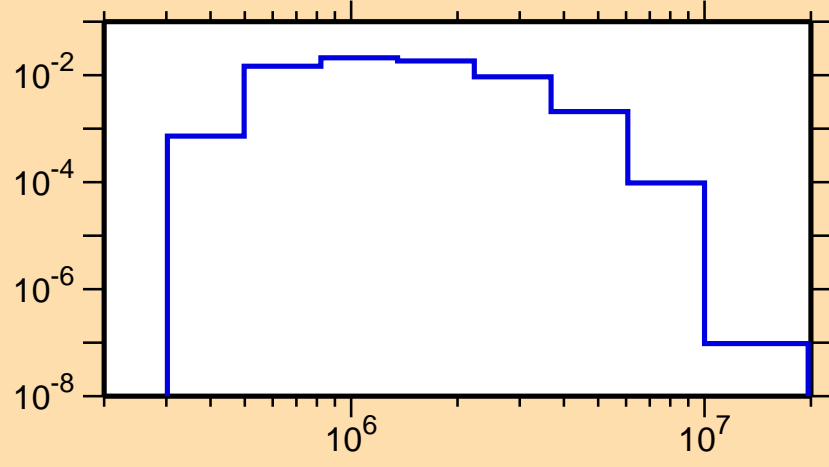
\sigma vs. E for ^{121}\text{Te}(n,n_3)
