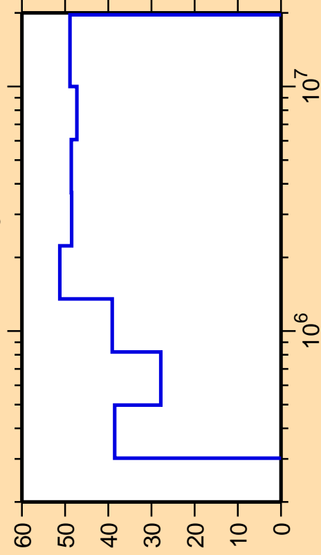
\Delta\sigma/\sigma vs. E for ^{121}\text{Te}(n,n_3)
