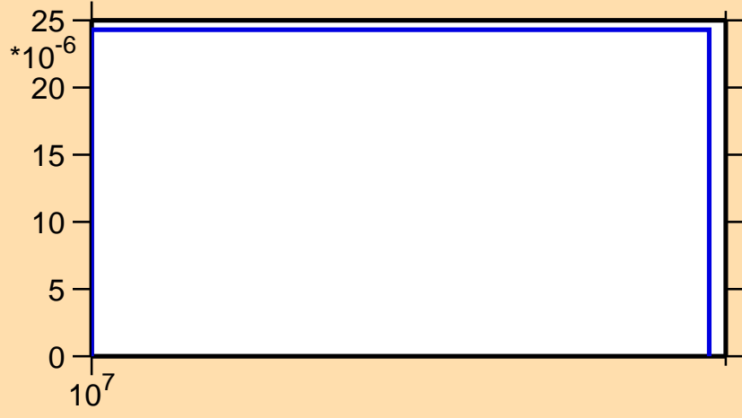
\sigma vs. E for ^{121}\text{Te}(n,3n)
