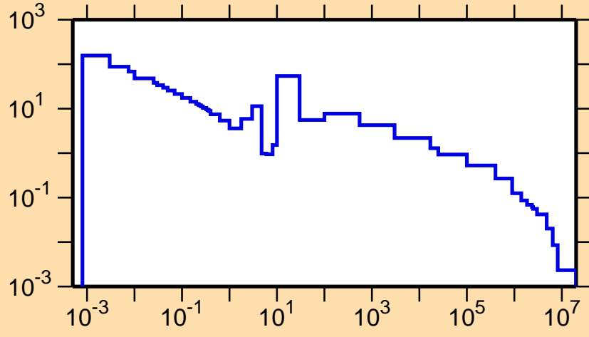
\sigma vs. E for ^{121}\text{Te}(n,\gamma)
