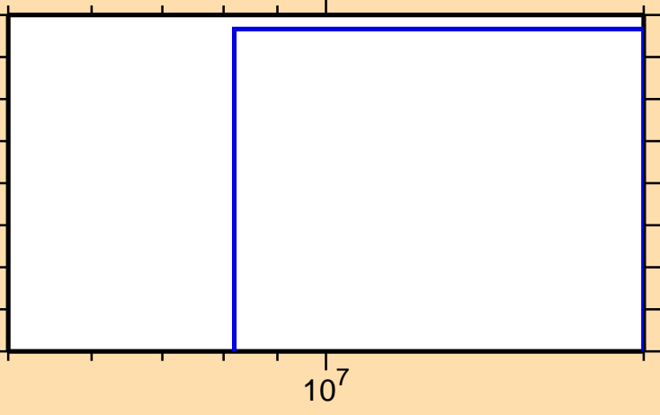
\sigma vs. E for ^{121}\text{Te}(n,\text{He3})
