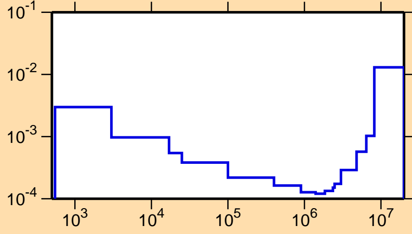
\sigma vs. E for ^{121}\text{Te}(n,\alpha)
