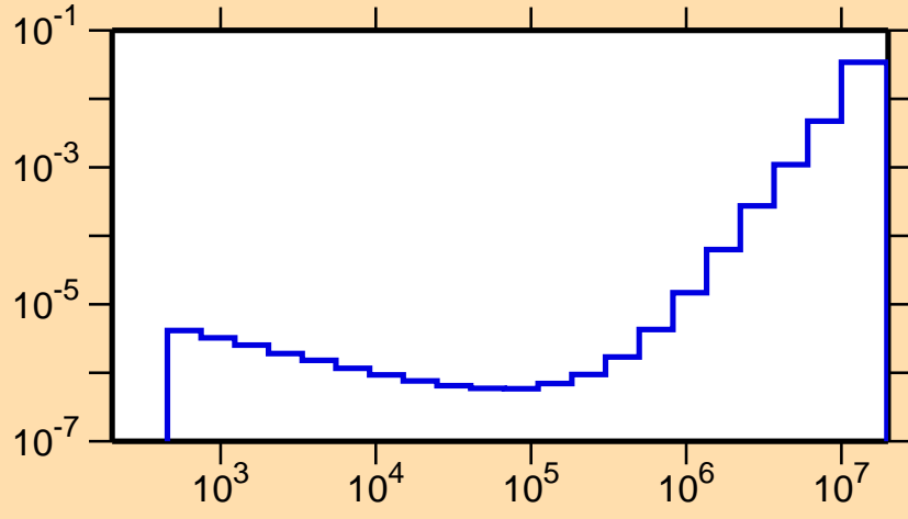
\sigma vs. E for ^{121}\text{Te}(n,p)
