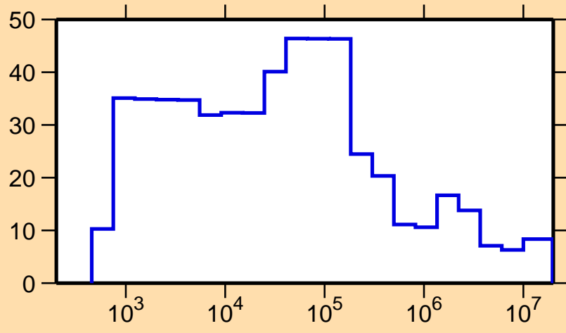
\Delta\sigma/\sigma vs. E for ^{121}\text{Te}(n,el.)
