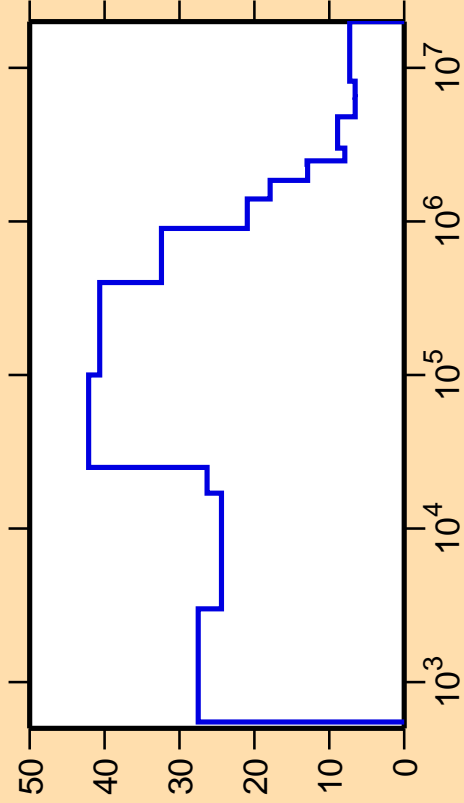
\Delta\sigma/\sigma vs. E for ^{121}\text{Te}(n,\text{nonel.})
