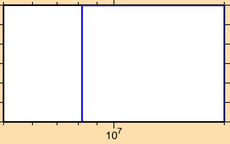
\sigma vs. E for ^{121}\text{Te}(n,t)
