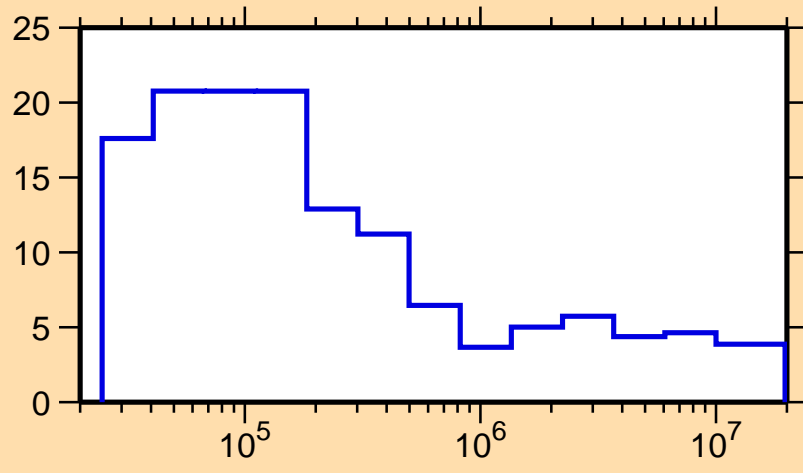
\Delta\sigma/\sigma vs. E for ^{122}\text{Te}(n,\text{tot.})
