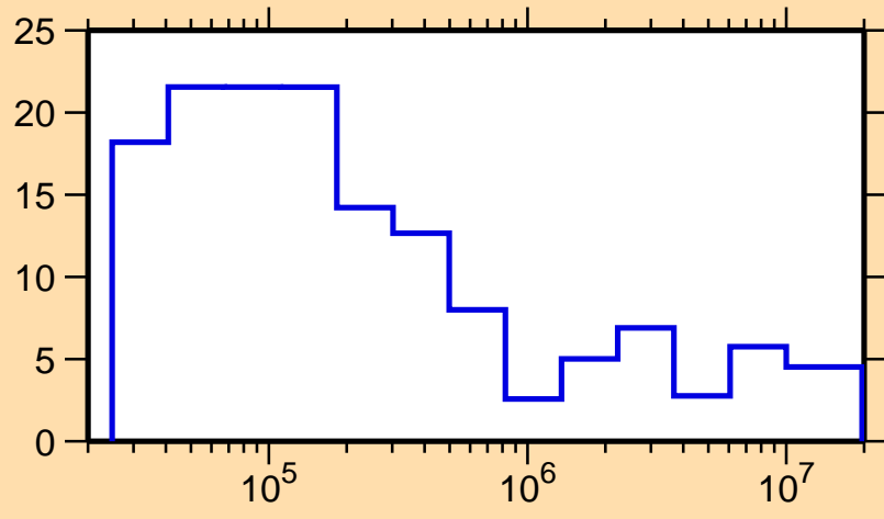
\Delta\sigma/\sigma vs. E for ^{122}\text{Te}(n,\text{el.})
