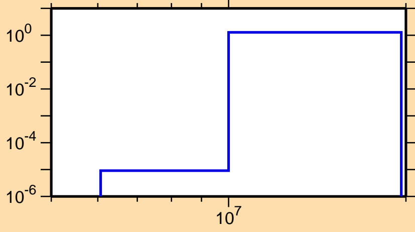
\sigma vs. E for ^{122}\text{Te}(n,2n)
