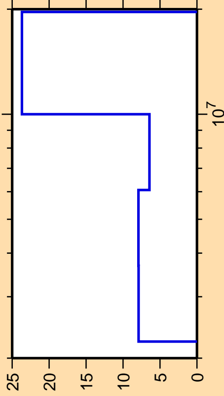
\Delta\sigma/\sigma vs. E for ^{122}\text{Te}(n,n\text{cont.})
