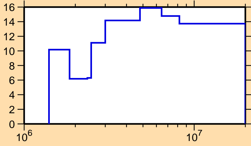
\Delta\sigma/\sigma vs. E for ^{122}\text{Te}(n,n_1)
