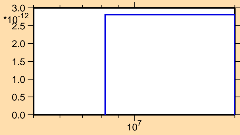
\sigma vs. E for ^{122}\text{Te}(n,2np)
