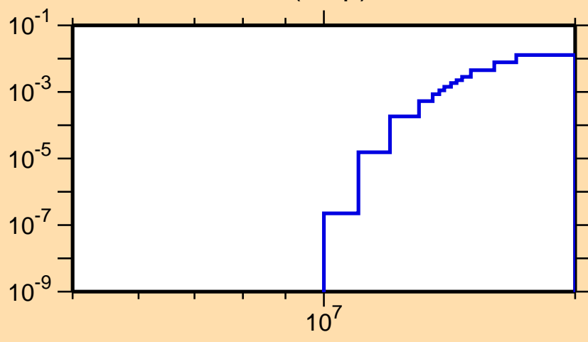
\sigma vs. E for ^{123}\text{Te}(n,np)
