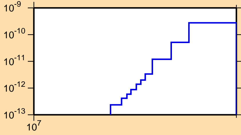
\sigma vs. E for ^{123}\text{Te}(n,p\alpha)
