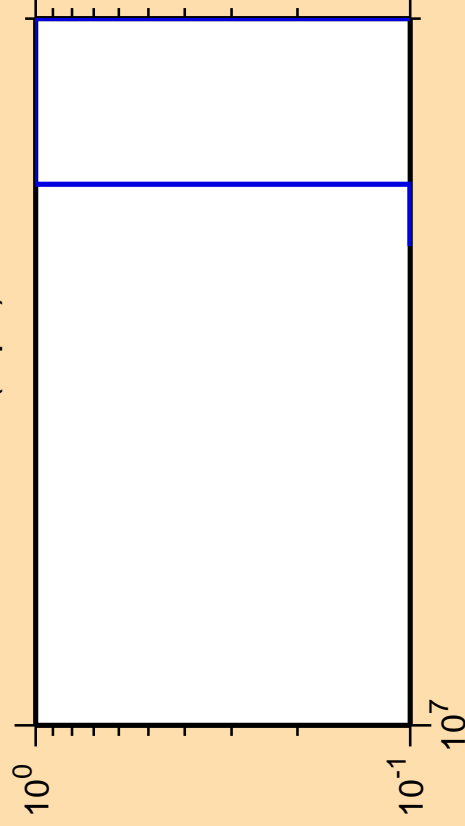
\Delta\sigma/\sigma vs. E for ^{123}\text{Te}(n,pd)
