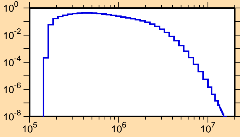
\sigma vs. E for ^{123}\text{Te}(n,n_1)
