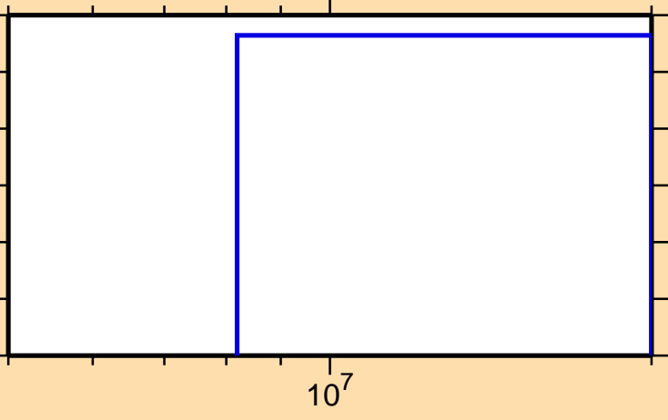
\sigma vs. E for ^{123}\text{Te} (mt 34)
