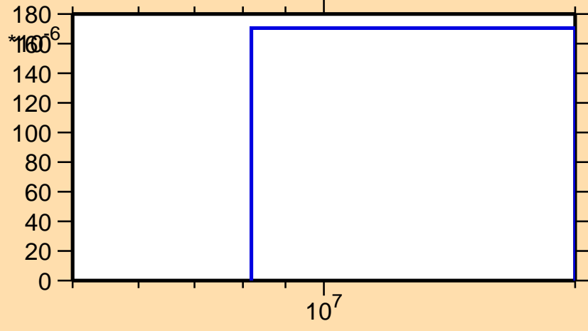
\sigma vs. E for ^{123}\text{Te}(n,t)
