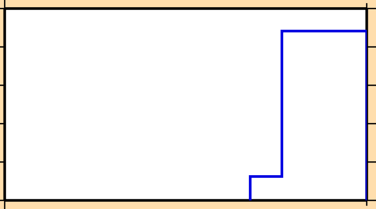
\sigma vs. E for ^{123}\text{Te}(n,pd)
