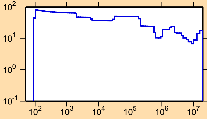
\Delta\sigma/\sigma vs. E for ^{123}\text{Te}(n,el.)
