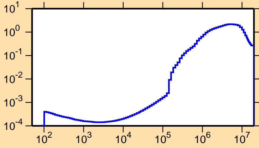
\sigma vs. E for ^{123}\text{Te}(n,\text{inel.})
