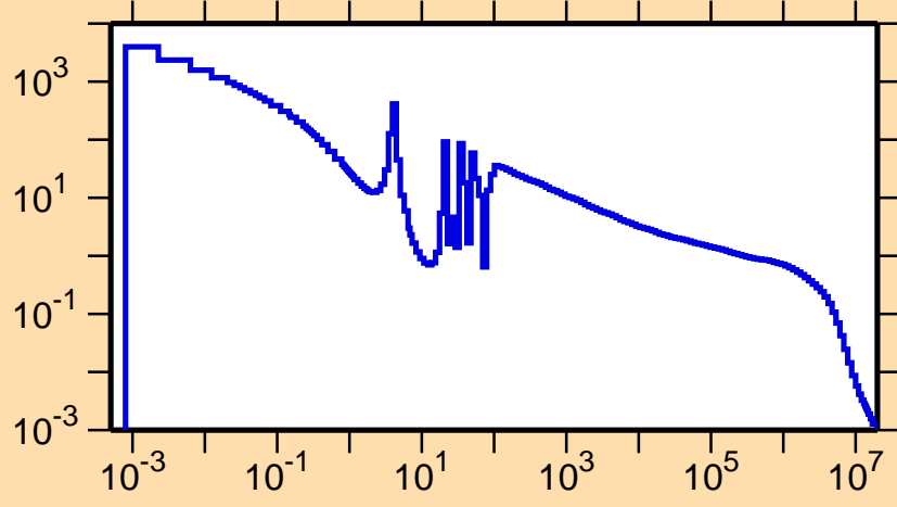
\sigma vs. E for ^{123}\text{Te}(n,\gamma)
