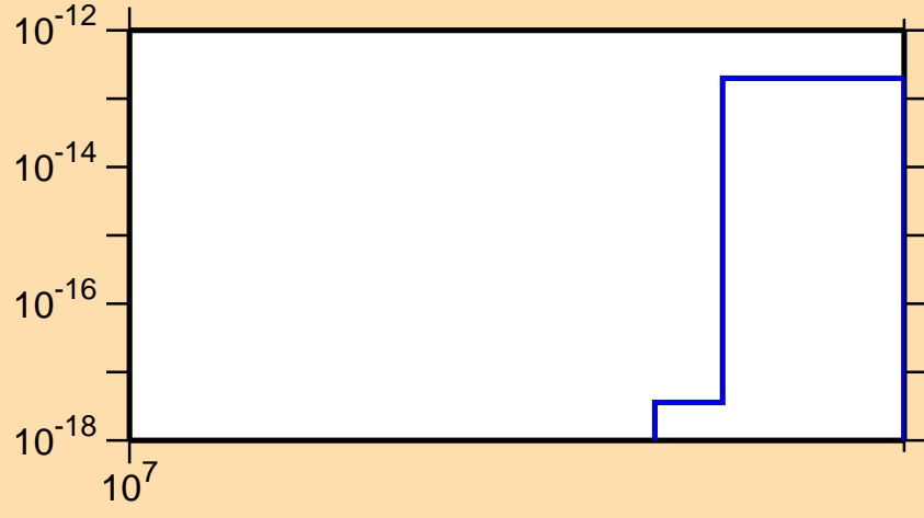
\sigma vs. E for ^{124}\text{Te}(n,pd)
