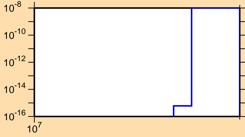
\sigma vs. E for ^{124}\text{Te}(n,\text{nd})
