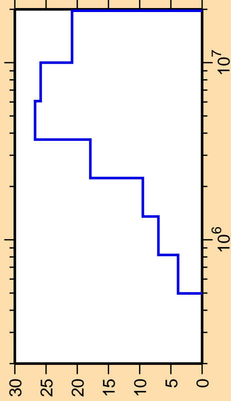
\Delta\sigma/\sigma vs. E for ^{124}\text{Te}(n,n_1)
