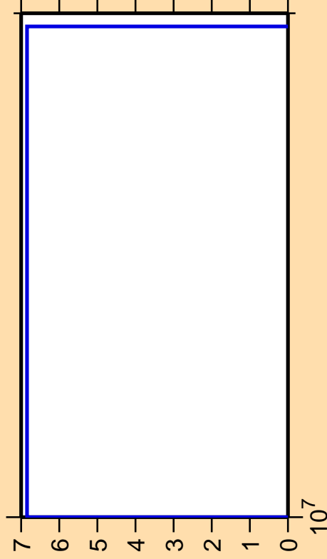
\Delta\sigma/\sigma vs. E for ^{124}\text{Te}(n,nt)
