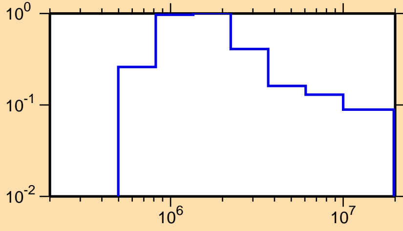
\sigma vs. E for ^{124}\text{Te}(n,n_1)
