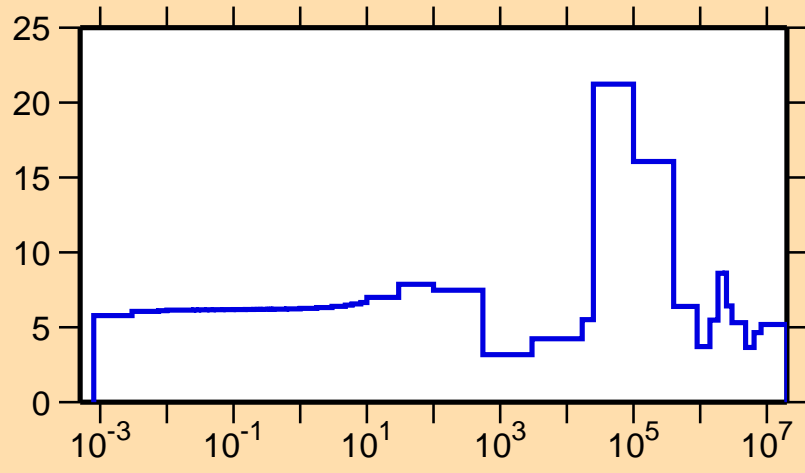
\Delta\sigma/\sigma vs. E for ^{124}\text{Te}(n,\text{el.})
