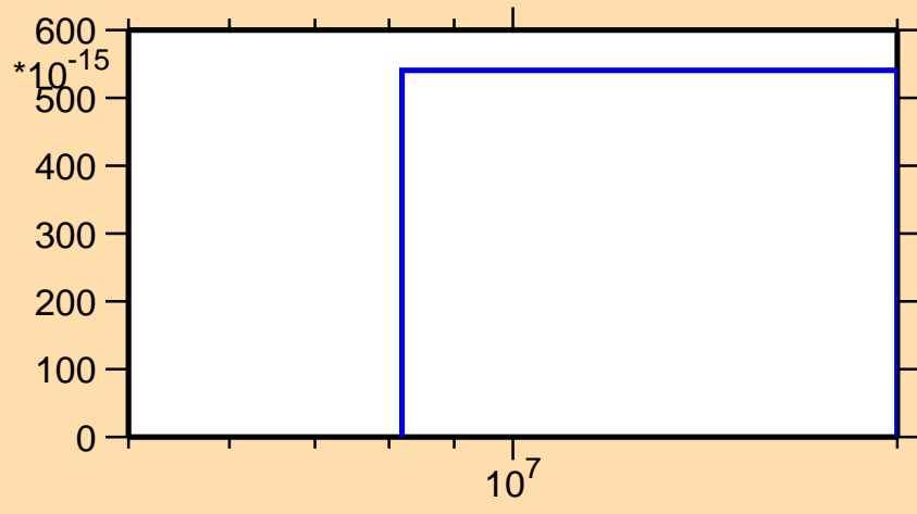
\sigma vs. E for ^{124}\text{Te}(n,2np)
