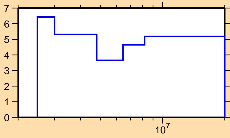
\Delta\sigma/\sigma vs. E for ^{124}\text{Te}(n,el.)
