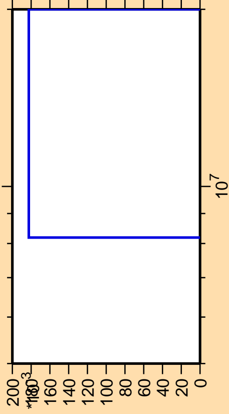
\Delta\sigma/\sigma vs. E for ^{124}\text{Te}(n,2np)
