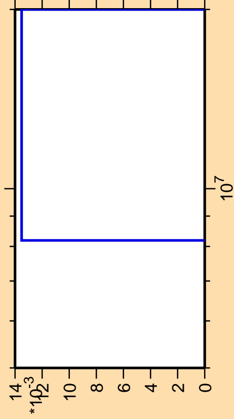
\Delta\sigma/\sigma vs. E for ^{124}\text{Te}(n,pd)
