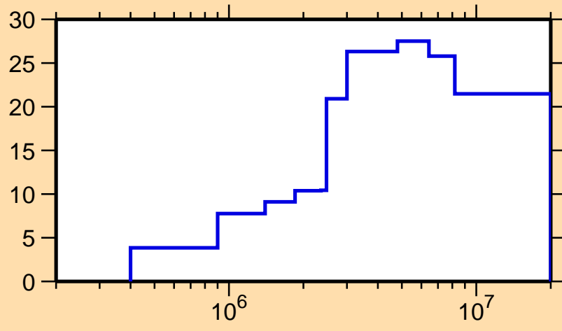
\Delta\sigma/\sigma vs. E for ^{124}\text{Te}(n,n_1)
