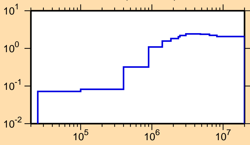
\sigma vs. E for ^{124}\text{Te}(n,\text{nonel.})
