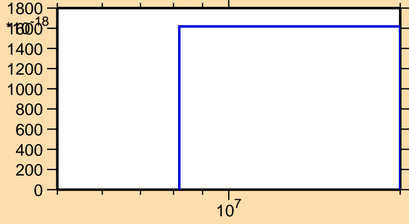
\sigma vs. E for ^{124}\text{Te}(n,pd)
