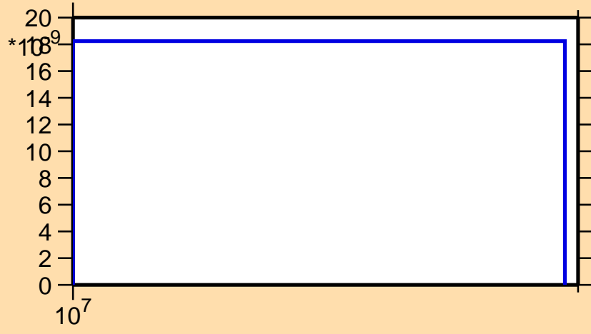
\sigma vs. E for ^{125}\text{Te}(n,2n\alpha)
