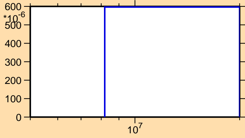
\sigma vs. E for ^{125}\text{Te}(n,d)
