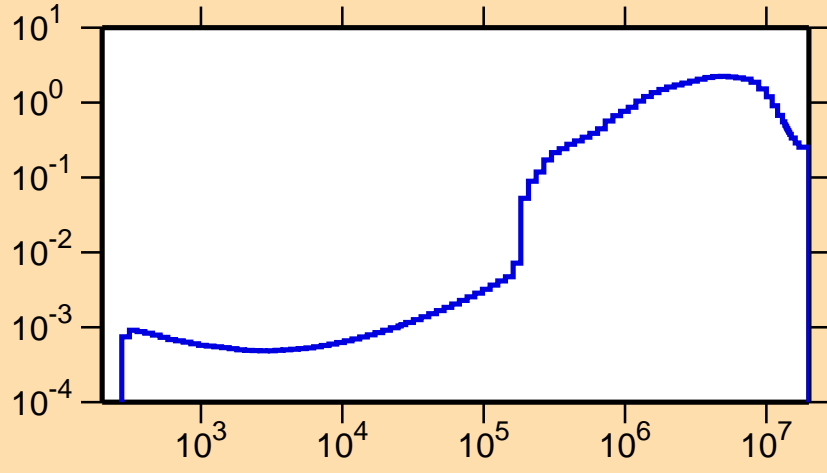
\sigma vs. E for ^{125}\text{Te}(n,\text{inel.})
