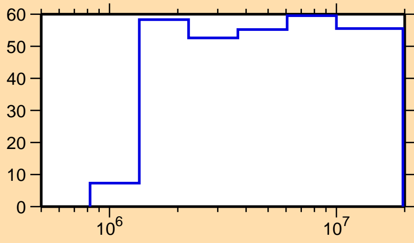
\Delta\sigma/\sigma vs. E for ^{125}\text{Te}(n,p)
