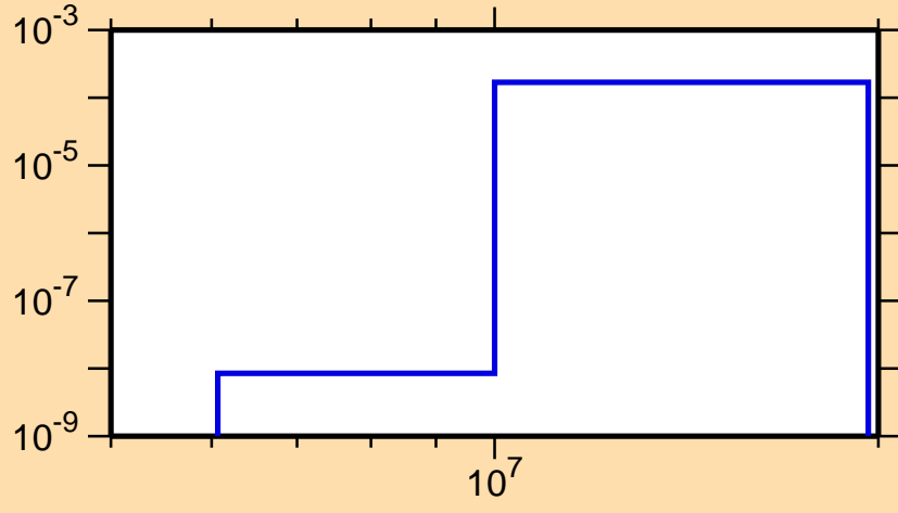
\sigma vs. E for ^{125}\text{Te}(n,n\alpha)
