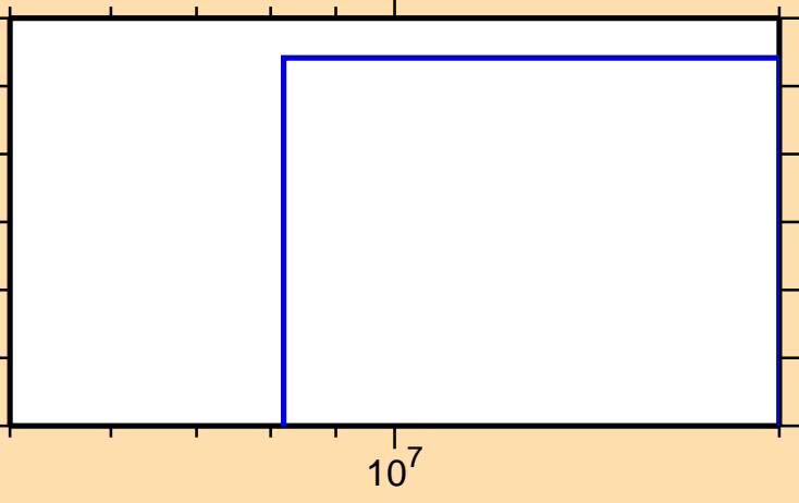
\sigma vs. E for ^{125}\text{Te}(n,2n\alpha)
