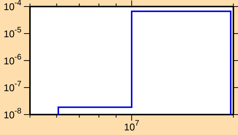
\sigma vs. E for ^{126}\text{Te}(n,n\alpha)
