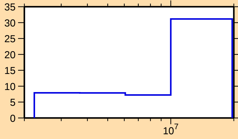
\Delta\sigma/\sigma vs. E for ^{126}\text{Te}(\text{n},\text{inel.})
