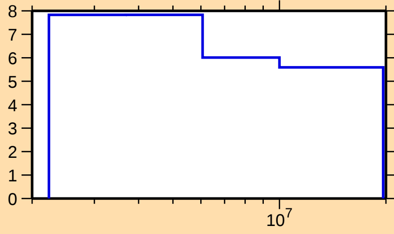
\Delta\sigma/\sigma vs. E for ^{126}\text{Te}(\text{n},\text{nonel.})
