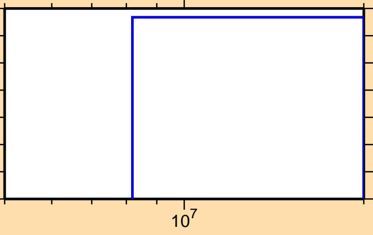
\sigma vs. E for ^{127}\text{Te}(n,nt)
