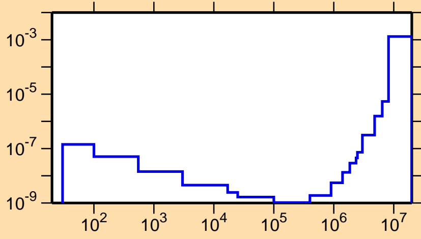
\sigma vs. E for ^{127}\text{Te}(n,\alpha)
