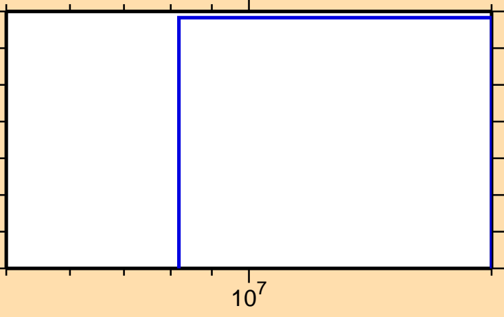
\sigma vs. E for ^{127}\text{Te}(n,2np)
