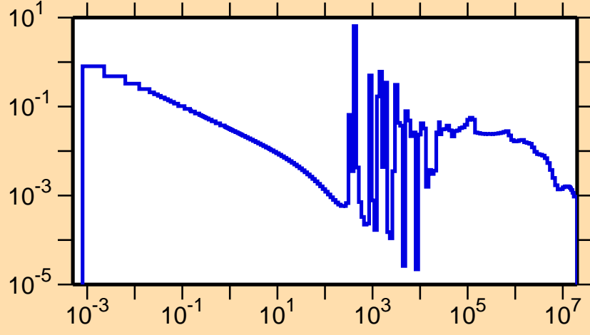
\sigma vs. E for ^{128}\text{Te}(n,\gamma)
