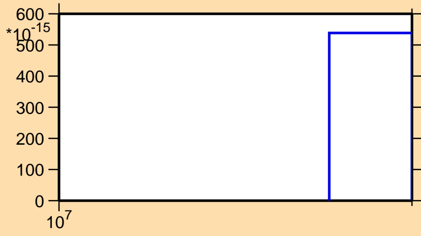
\sigma vs. E for ^{128}\text{Te}(n,2np)
