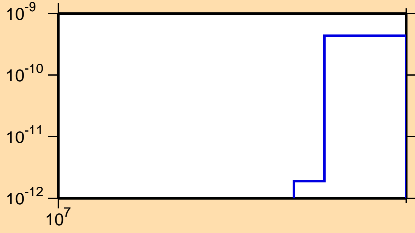
\sigma vs. E for ^{128}\text{Te}(n,2n\alpha)
