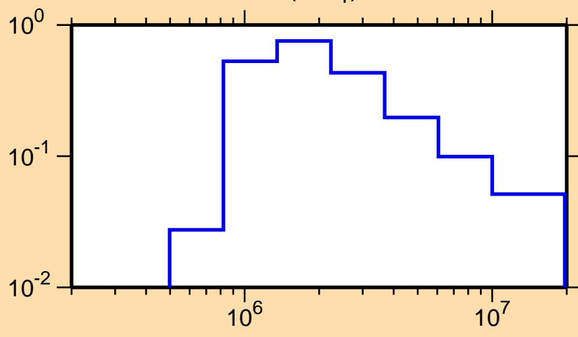
\sigma vs. E for ^{128}\text{Te}(n,n_1)
