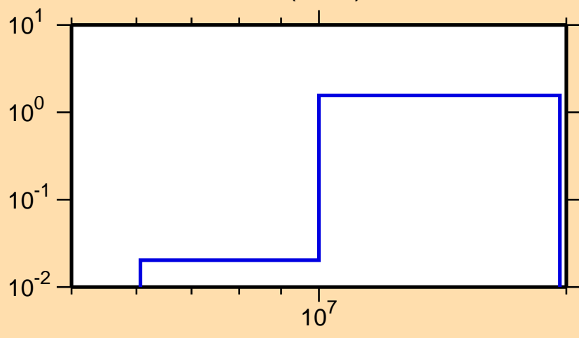
\sigma vs. E for ^{128}\text{Te}(n,2n)
