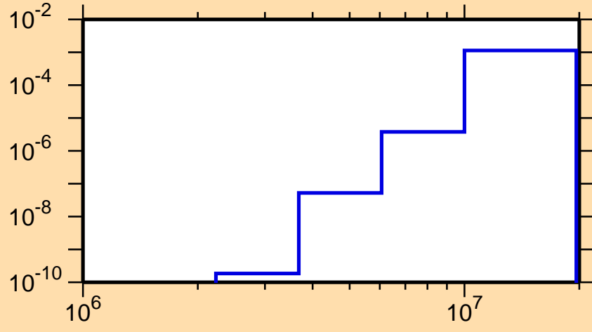
\sigma vs. E for ^{128}\text{Te}(n,\alpha)
