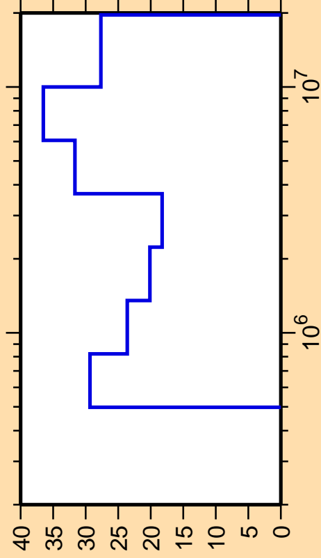
\Delta\sigma/\sigma vs. E for ^{128}\text{Te}(n,n_1)
