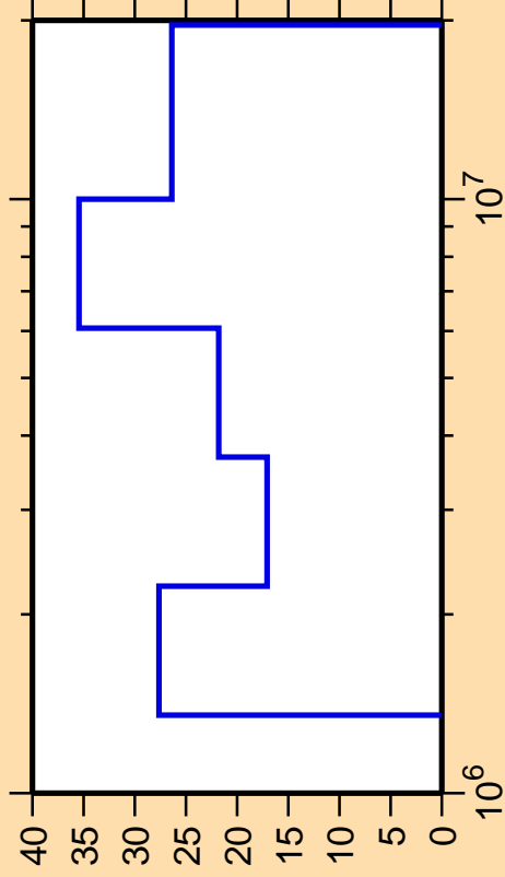
\Delta\sigma/\sigma vs. E for ^{128}\text{Te}(n,n_2)
