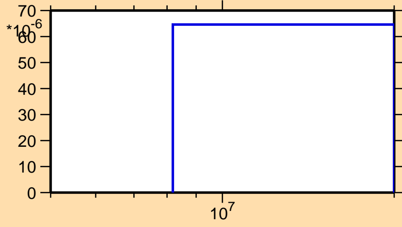
\sigma vs. E for ^{128}\text{Te}(n,np)
