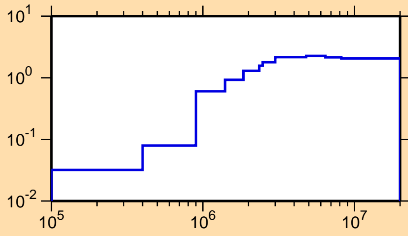
\sigma vs. E for ^{128}\text{Te}(n,\text{nonel.})
