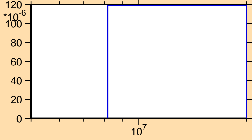
\sigma vs. E for ^{128}\text{Te}(n,d)
