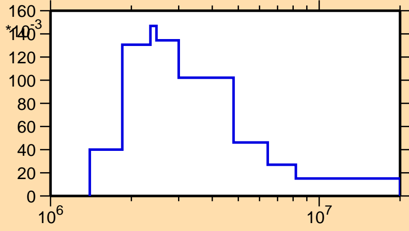
\sigma vs. E for ^{128}\text{Te}(n,n_2)
