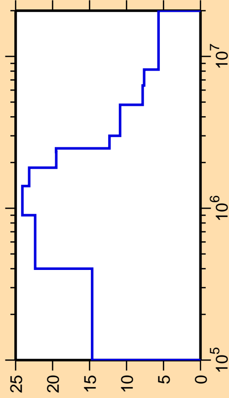
\Delta\sigma/\sigma vs. E for ^{128}\text{Te}(n,\text{nonel.})
