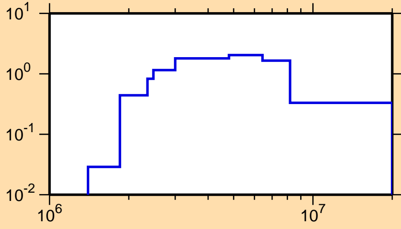
\sigma vs. E for ^{129}\text{Te}(n,n\text{cont.})
