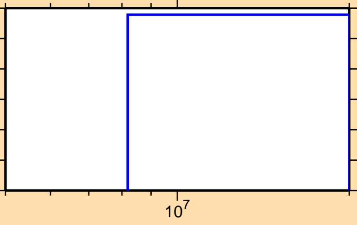
\sigma vs. E for ^{129}\text{Te}(n,3n)
