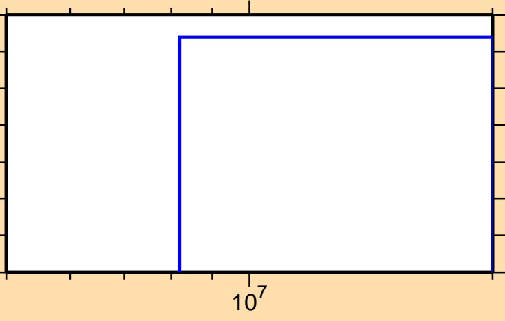
\sigma vs. E for ^{129}\text{Te}(n,d)
