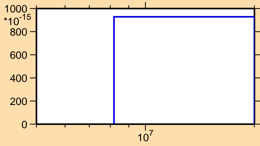
\sigma vs. E for ^{130}\text{Te}(n,2n\alpha)
