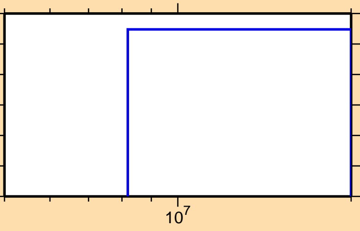
\sigma vs. E for ^{130}\text{Te}(n,\text{He3})
