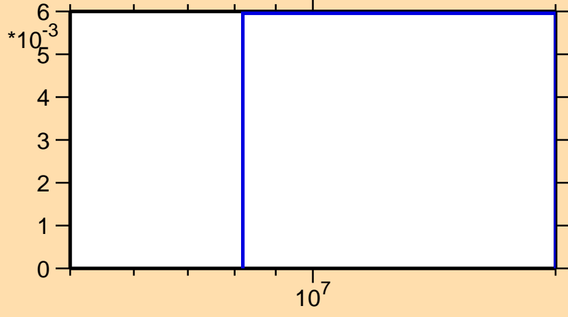
\sigma vs. E for ^{130}\text{Te}(n,3n)
