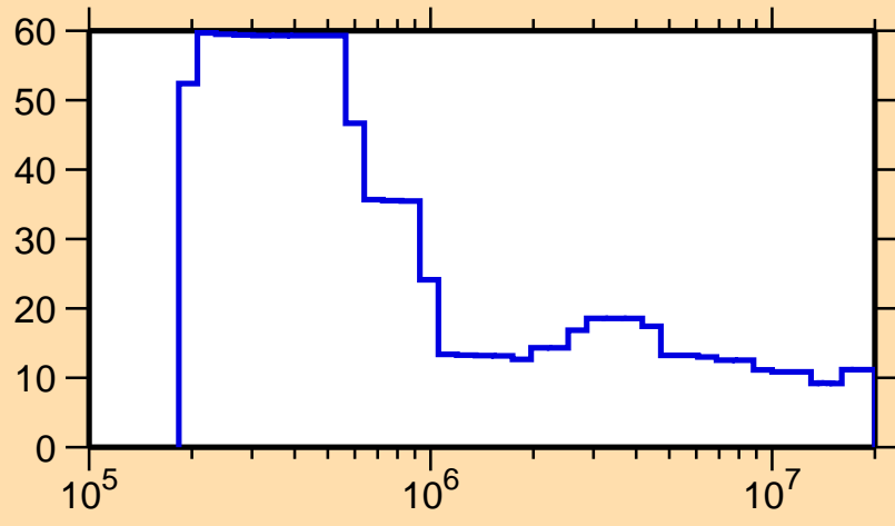
\Delta\sigma/\sigma vs. E for ^{131}\text{Te}(n,\text{nonel.})
