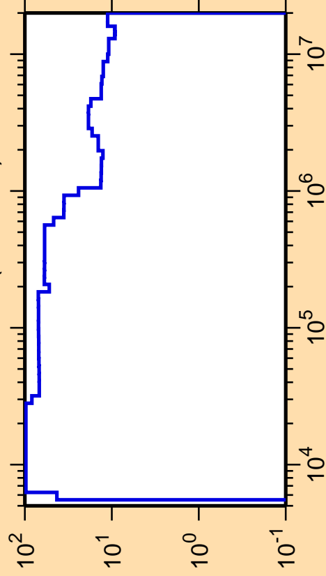
\Delta\sigma/\sigma vs. E for ^{131}\text{Te}(n,\text{nonel.})
