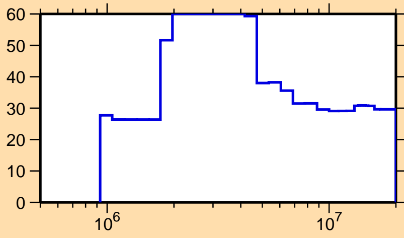
\Delta\sigma/\sigma vs. E for ^{131}\text{Te}(n,n_1)
