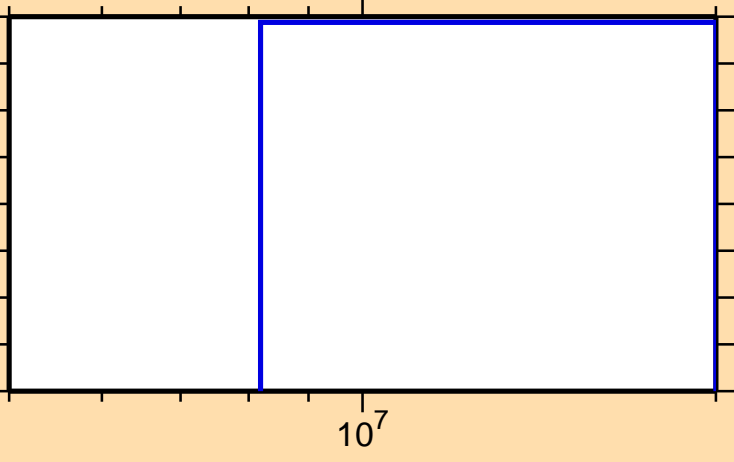
\sigma vs. E for ^{131}\text{Te}(n,\text{He3})
