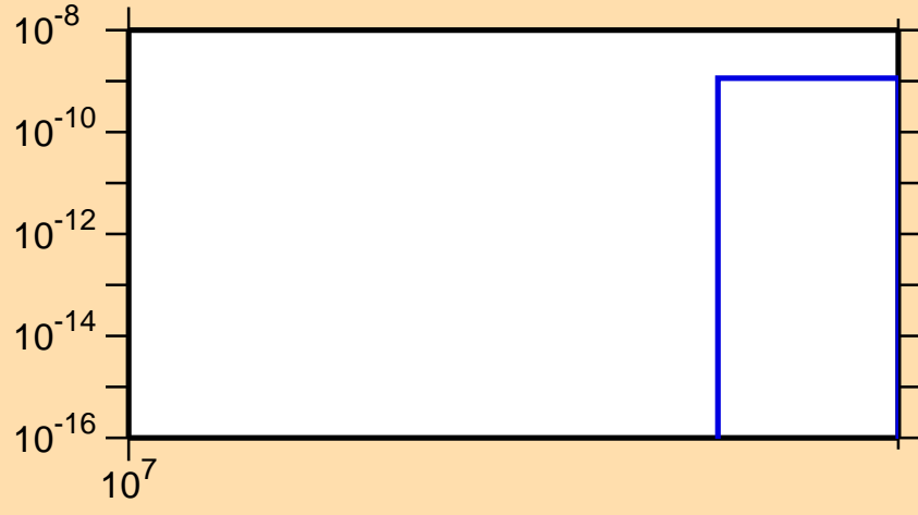
\sigma vs. E for ^{131}\text{Te}(n,nt)
