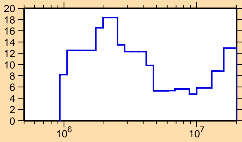
\Delta\sigma/\sigma vs. E for ^{131}\text{Te}(n,\text{tot.})
