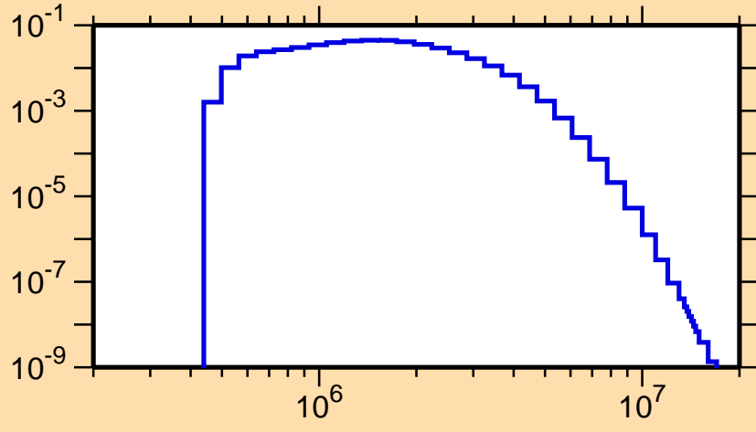
\sigma vs. E for ^{131}\text{Te}(n,n_3)
