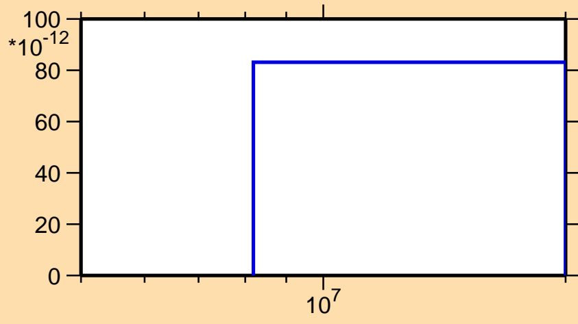
\sigma vs. E for ^{131}\text{Te}(n,2np)
