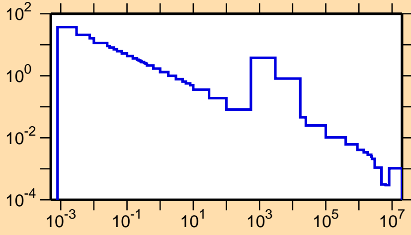
\sigma vs. E for ^{131}\text{Te}(n,\gamma)
