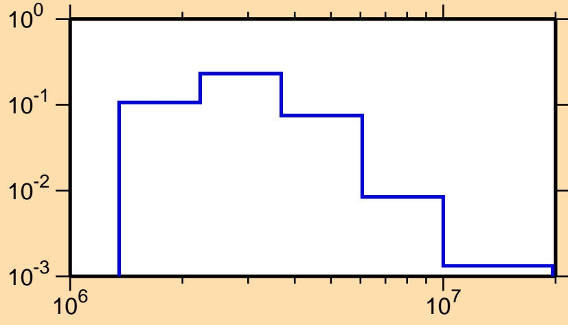
\sigma vs. E for ^{132}\text{Te}(n,n_2)
