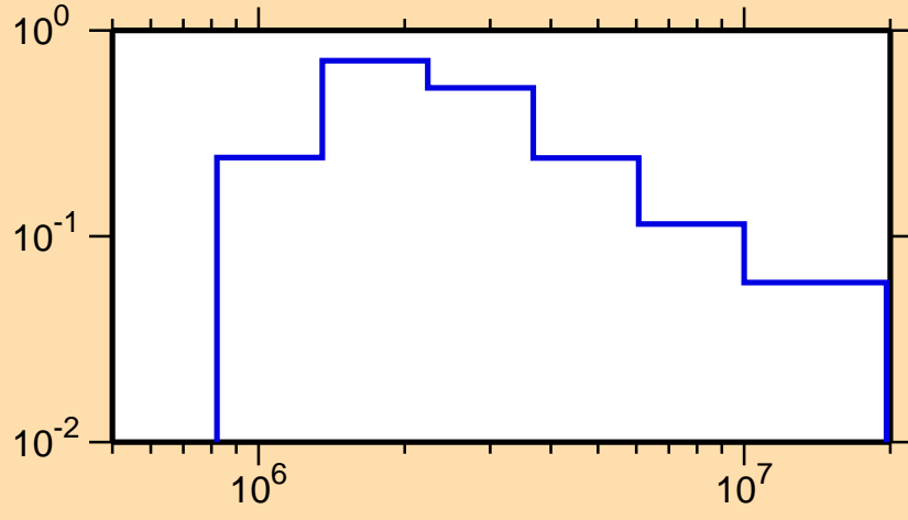
\sigma vs. E for ^{132}\text{Te}(n,n_1)
