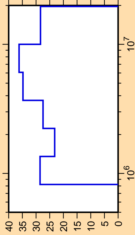
\Delta\sigma/\sigma vs. E for ^{132}\text{Te}(n,n_1)
