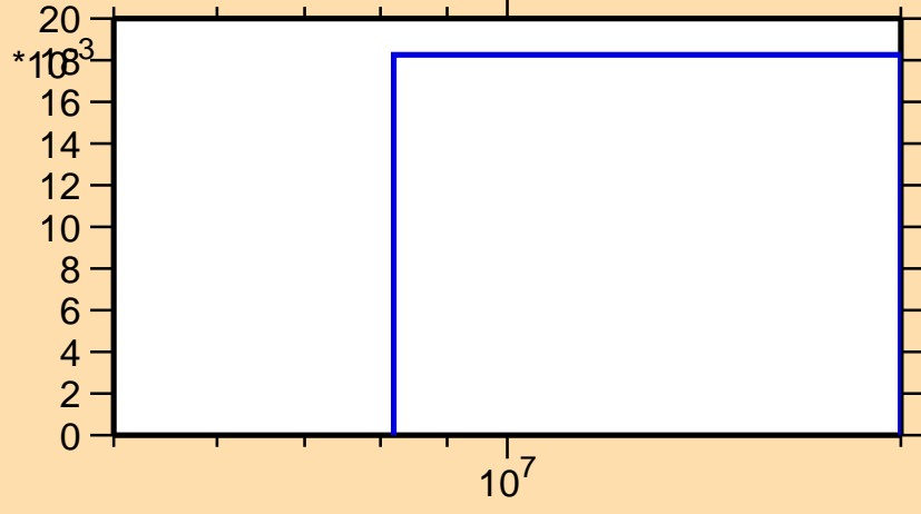
\sigma vs. E for ^{132}\text{Te}(n,3n)
