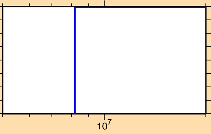
\sigma vs. E for ^{132}\text{Te}(n,nt)
