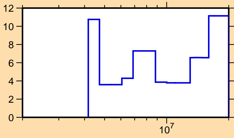
\Delta\sigma/\sigma vs. E for ^{133}\text{Te}(n,el.)
