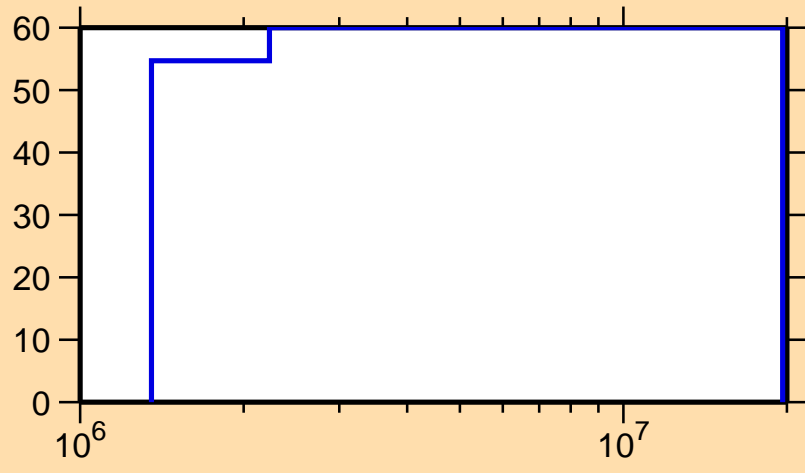
\Delta\sigma/\sigma vs. E for ^{133}\text{Te}(n,\gamma)
