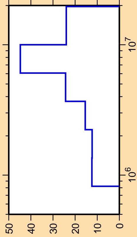
\Delta\sigma/\sigma vs. E for ^{133}\text{Te}(n,n_3)
