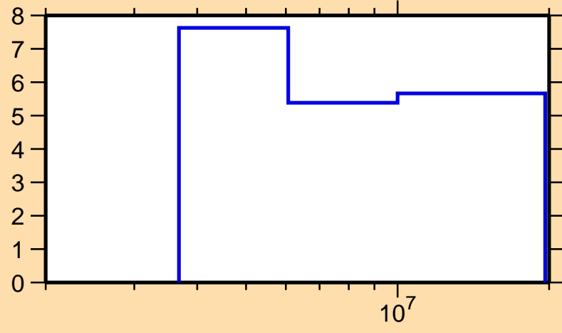
\Delta\sigma/\sigma vs. E for ^{133}\text{Te}(n,el.)
