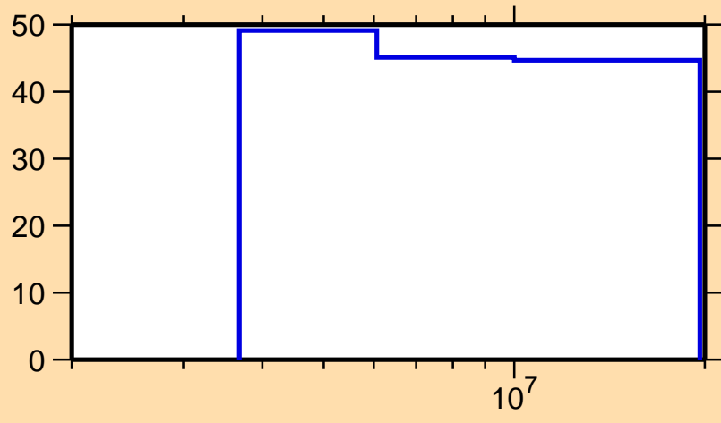
\Delta\sigma/\sigma vs. E for ^{133}\text{Te}(n,p)
