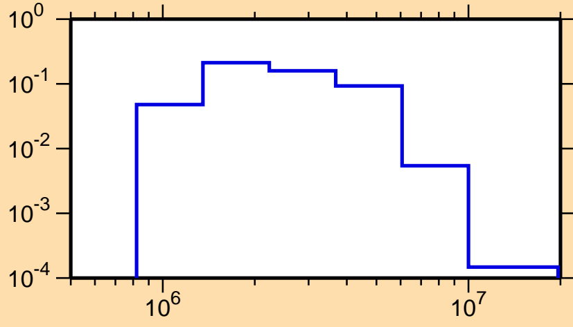
\sigma vs. E for ^{133}\text{Te}(n,n_3)
