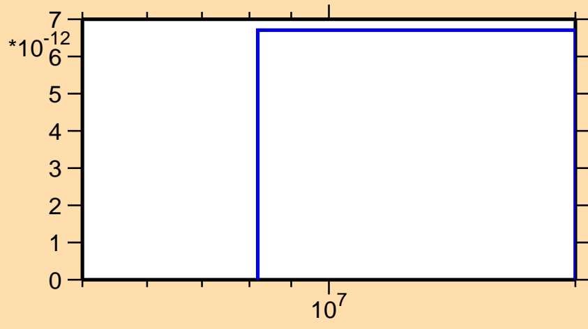
\sigma vs. E for ^{133}\text{Te}(n,nt)
