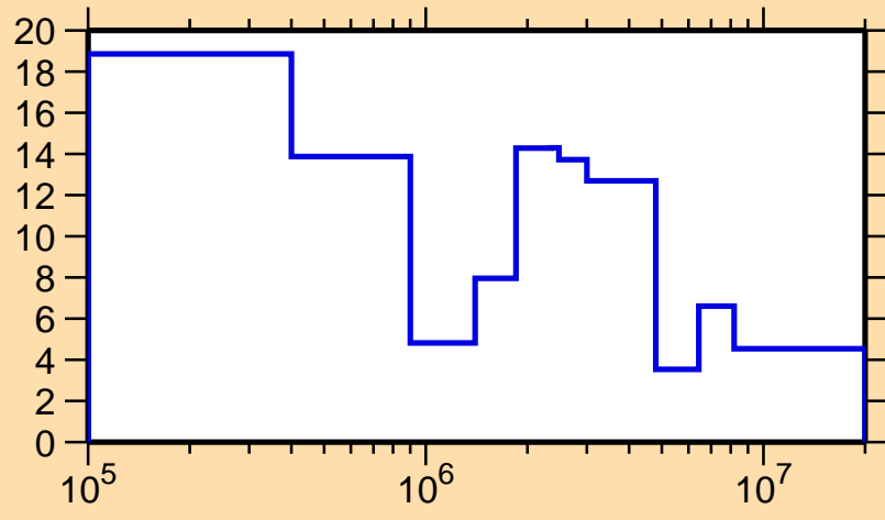
\Delta\sigma/\sigma vs. E for ^{133}\text{Te}(n,\text{el.})
