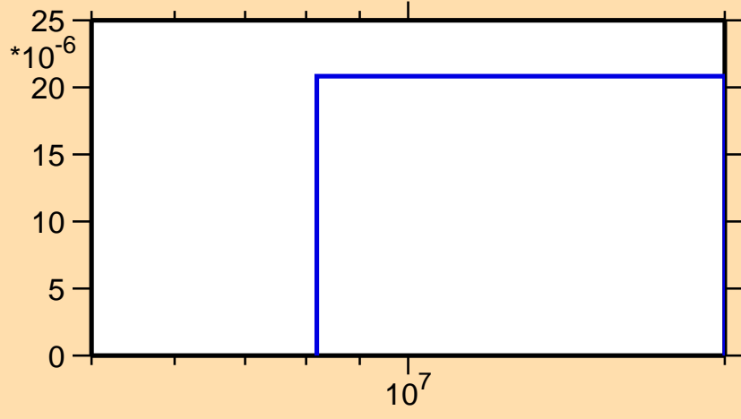
\sigma vs. E for ^{133}\text{Te}(n,np)
