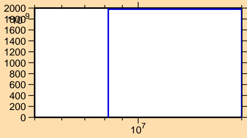
\sigma vs. E for ^{133}\text{Te}(n,n\alpha)
