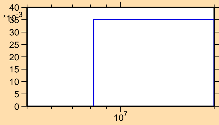
\sigma vs. E for ^{133}\text{Te}(n,3n)
