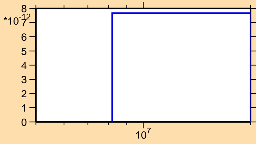
\sigma vs. E for ^{133}\text{Te}(n,2np)
