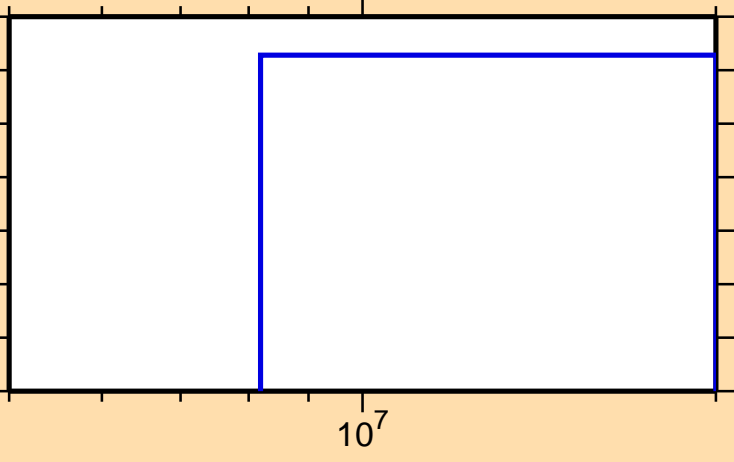
\sigma vs. E for ^{133}\text{Te}(n,d)
