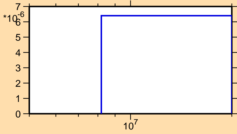
\sigma vs. E for ^{133}\text{Te}(n,t)
