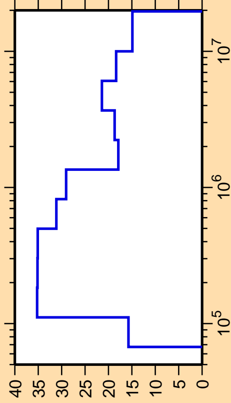
\Delta\sigma/\sigma vs. E for ^{133}\text{Te}(n,\text{nonel.})
