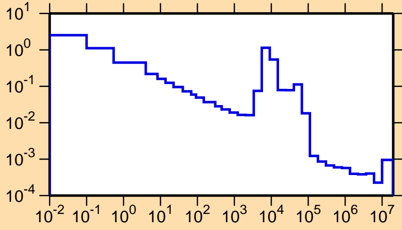
\sigma vs. E for ^{133}\text{Te}(n,\gamma)
