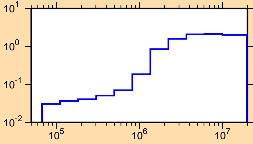
\sigma vs. E for ^{133}\text{Te}(n,\text{nonel.})
