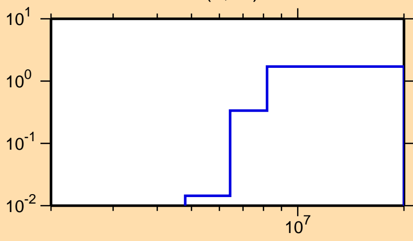
\sigma vs. E for ^{133}\text{Te}(n,2n)
