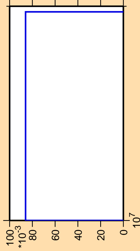
\Delta\sigma/\sigma vs. E for ^{134}\text{Te}(n,2n\alpha)
