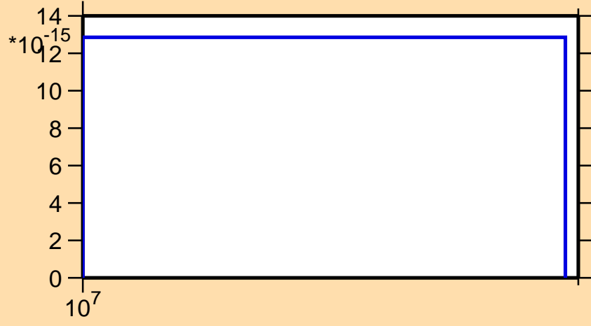
\sigma vs. E for ^{134}\text{Te}(n,2n\alpha)
