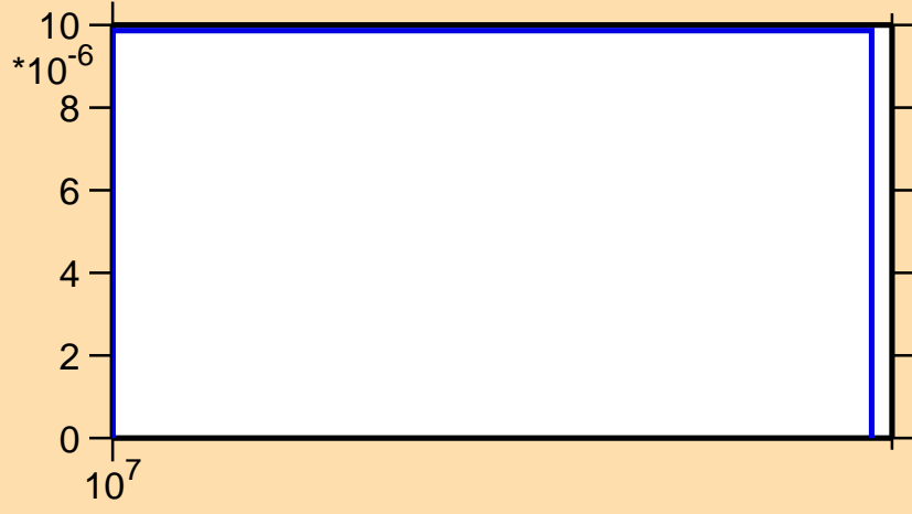
\sigma vs. E for ^{134}\text{Te}(n,np)
