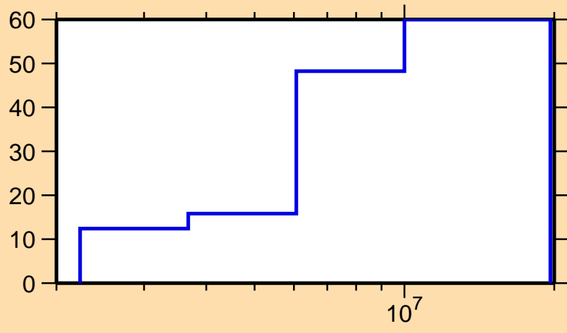
\Delta\sigma/\sigma vs. E for ^{134}\text{Te}(n,n_1)
