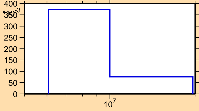
\sigma vs. E for ^{134}\text{Te}(n,n\text{cont.})
