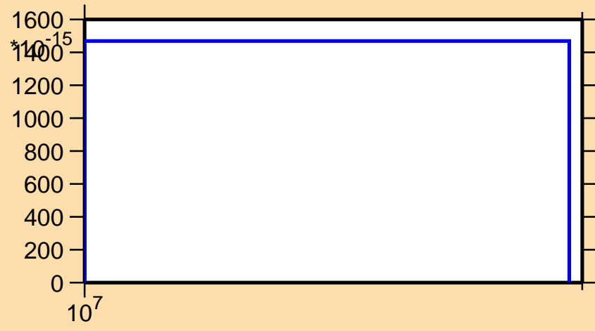
\sigma vs. E for ^{134}\text{Te}(n,nd)
