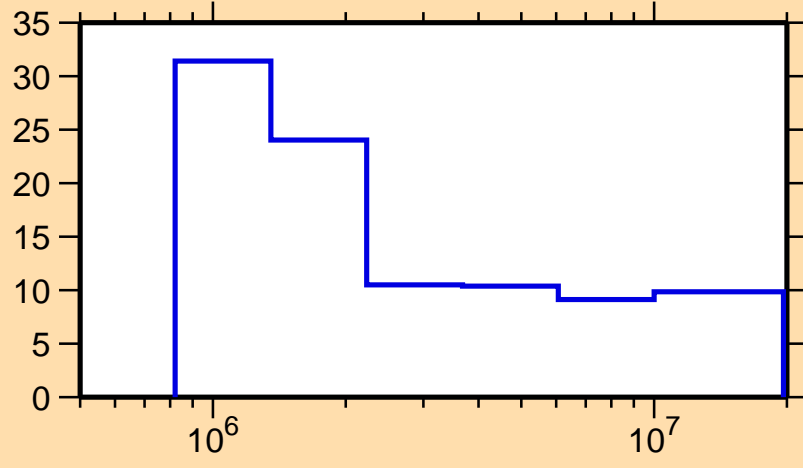
\Delta\sigma/\sigma vs. E for ^{134}\text{Te}(n,\text{nonel.})
