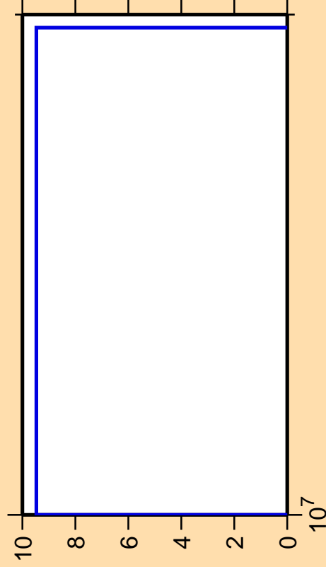
\Delta\sigma/\sigma vs. E for ^{134}\text{Te}(n,nd)
