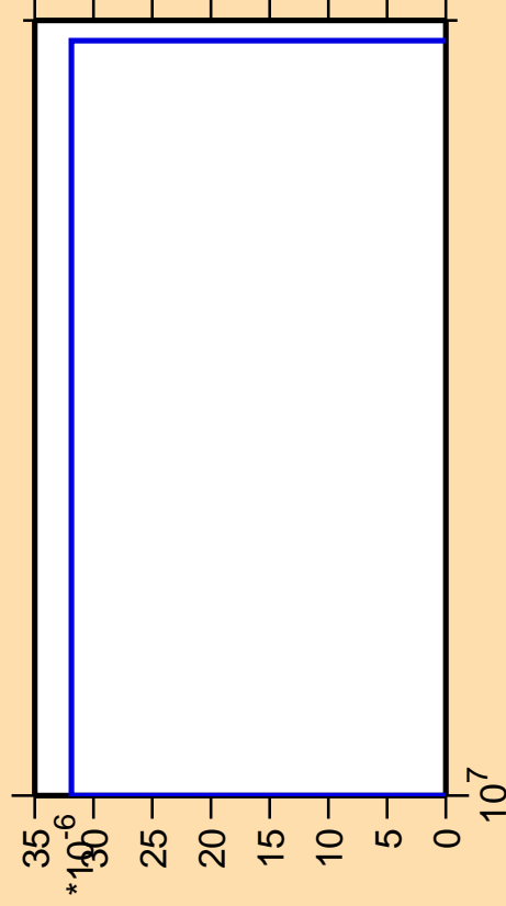
\Delta\sigma/\sigma vs. E for ^{134}\text{Te}(n,2np)
