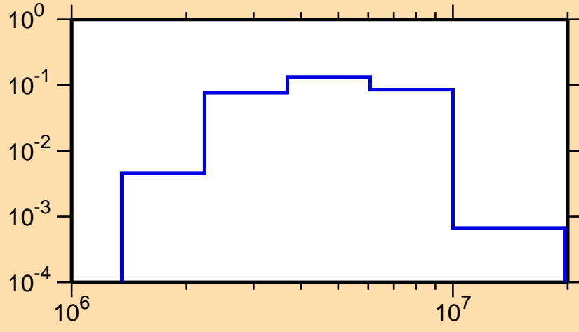
\sigma vs. E for ^{134}\text{Te}(n,n_3)
