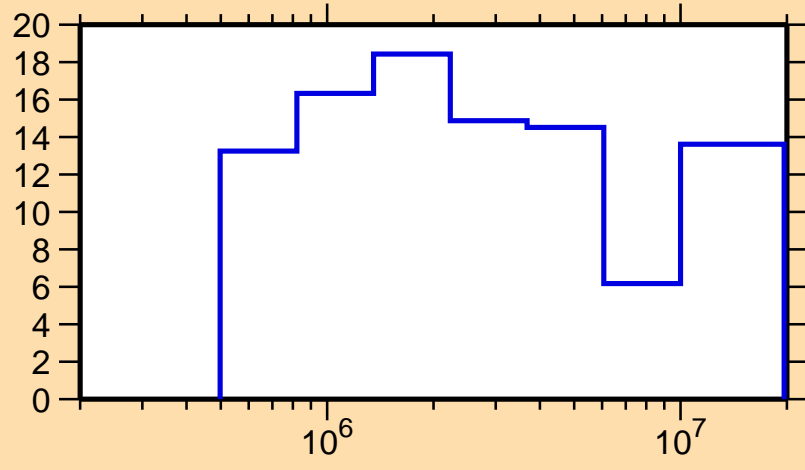
\Delta\sigma/\sigma vs. E for ^{134}\text{Te}(n,\text{tot.})
