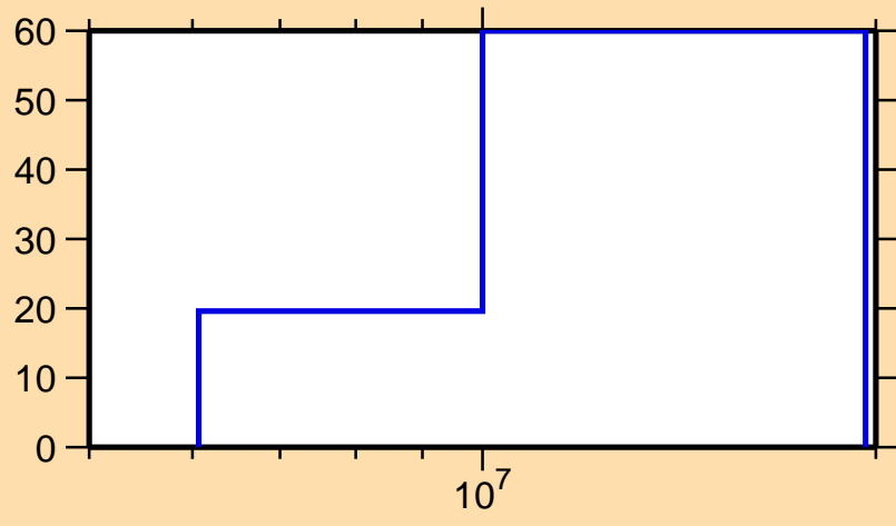
\Delta\sigma/\sigma vs. E for ^{134}\text{Te}(n,\text{inel.})
