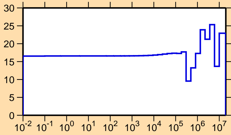
\Delta\sigma/\sigma vs. E for ^{134}\text{Te}(n,\text{el.})
