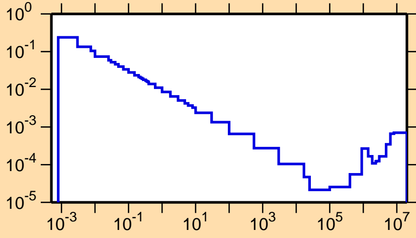
\sigma vs. E for ^{134}\text{Te}(n,\gamma)
