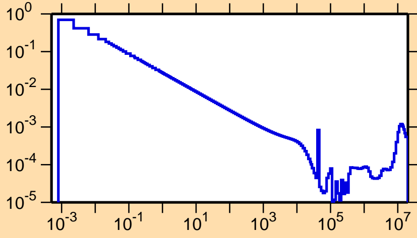
\sigma vs. E for ^{135}\text{Te}(n,\gamma)
