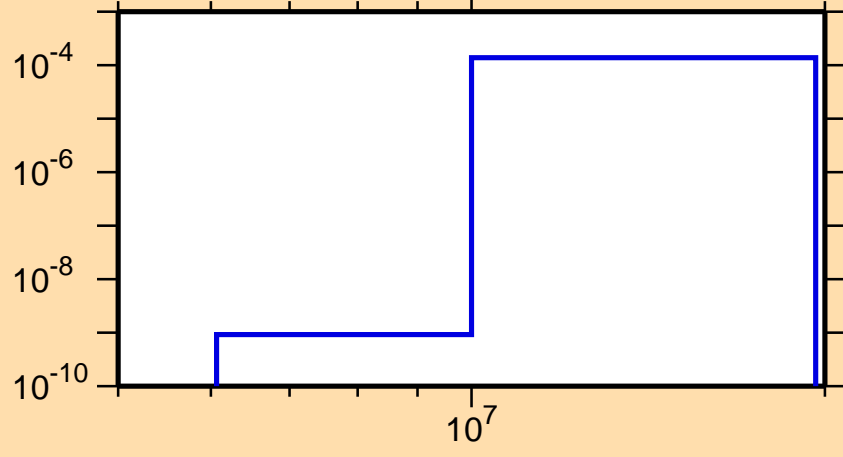
\sigma vs. E for ^{135}\text{Te}(n,t)
