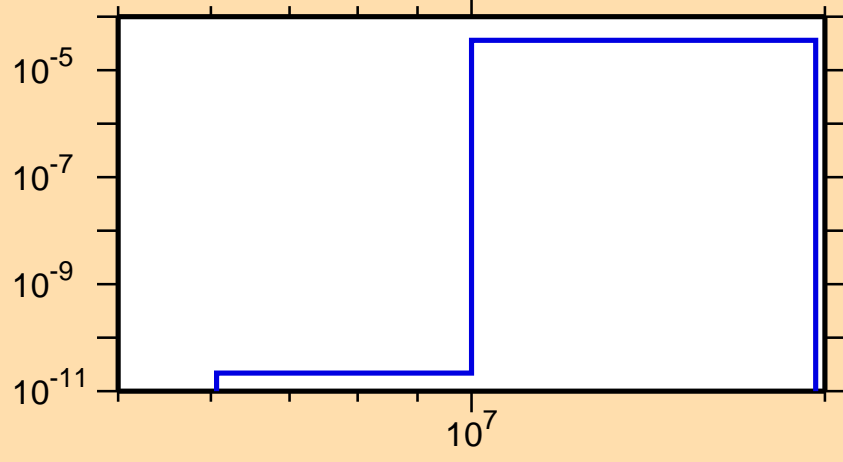
\sigma vs. E for ^{135}\text{Te}(n,\alpha)
