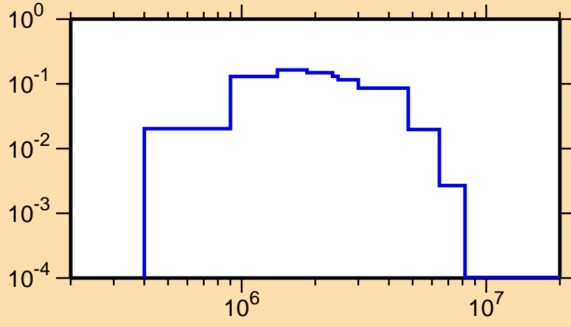
\sigma vs. E for ^{135}\text{Te}(n,n_1)
