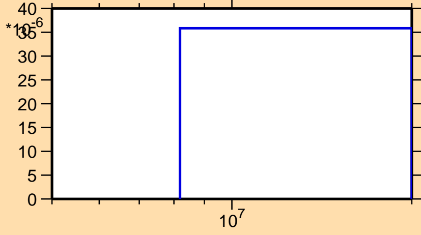
\sigma vs. E for ^{135}\text{Te}(n,d)
