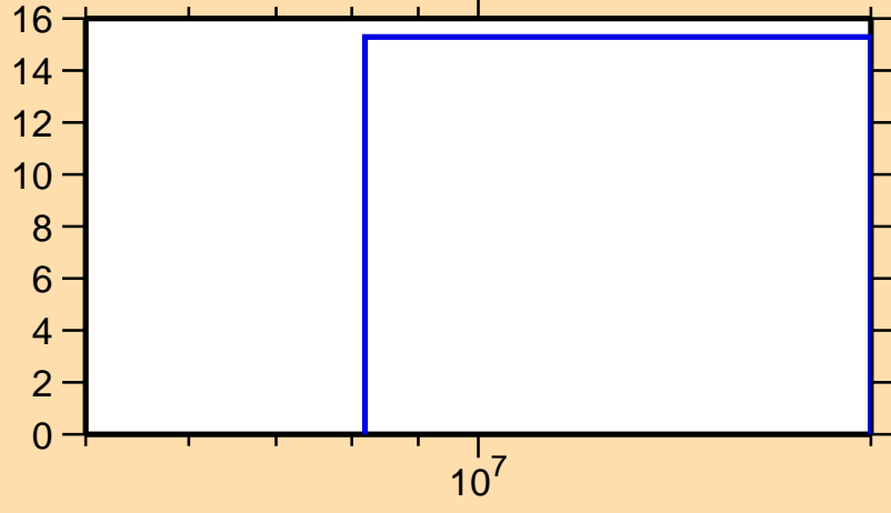
\Delta\sigma/\sigma vs. E for ^{135}\text{Te}(n,el.)
