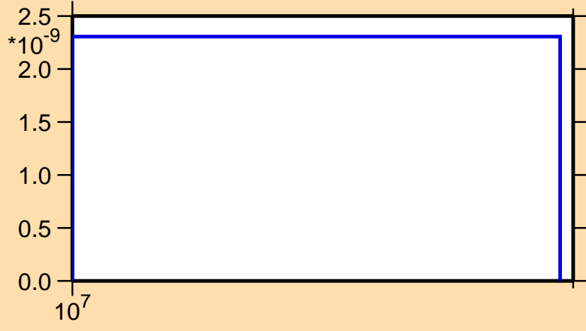
\sigma vs. E for ^{136}\text{Te}(n,2n\alpha)
