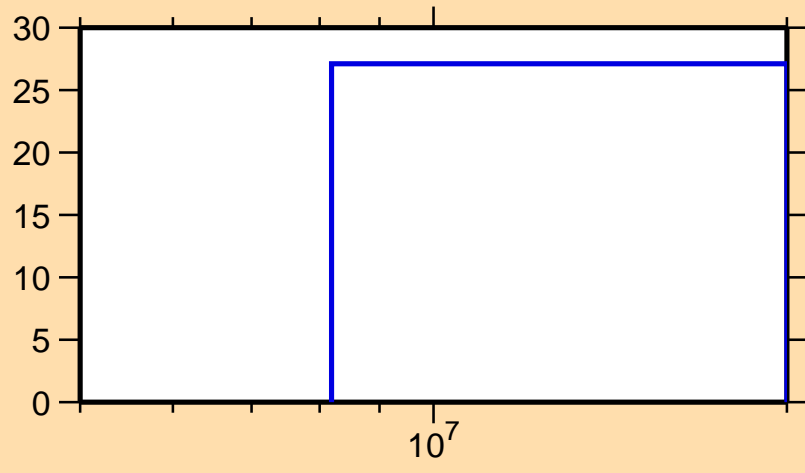
\Delta\sigma/\sigma vs. E for ^{136}\text{Te}(n,el.)
