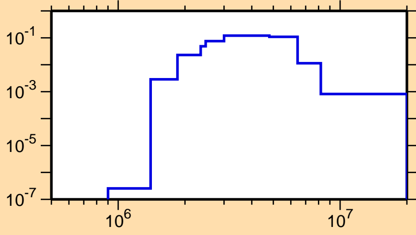
\sigma vs. E for ^{136}\text{Te}(n,n_3)
