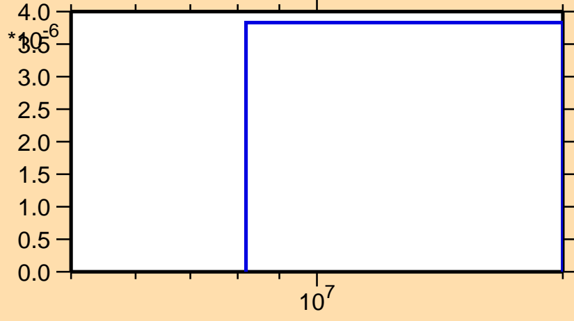
\sigma vs. E for ^{136}\text{Te}(n,d)
