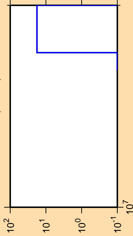
\Delta\sigma/\sigma vs. E for ^{137}\text{Te} (mt 11)
