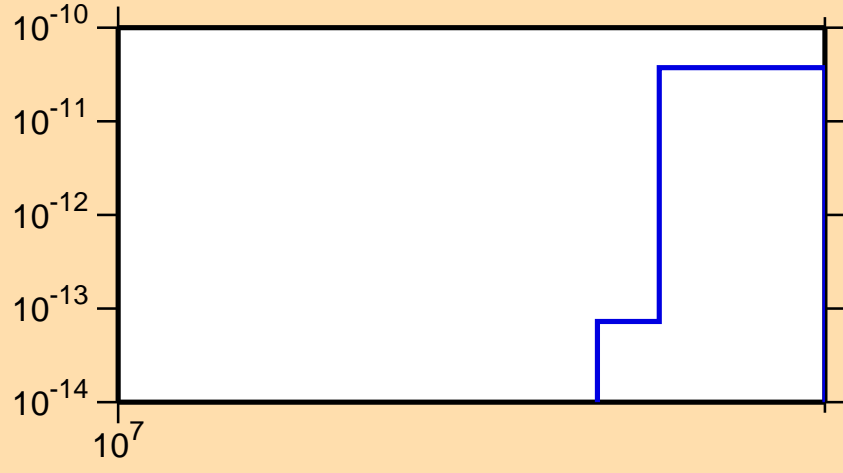
\sigma vs. E for ^{137}\text{Te}(n,3n\alpha)
