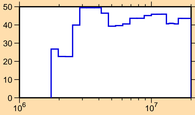
\Delta\sigma/\sigma vs. E for ^{137}\text{Te}(n,n_1)
