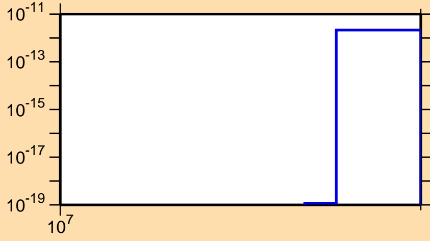
\sigma vs. E for ^{137}\text{Te} (mt 11)
