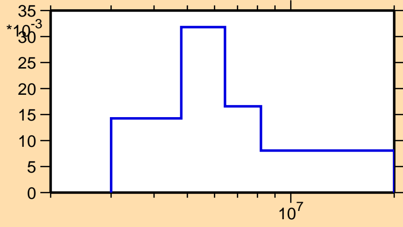
\sigma vs. E for ^{137}\text{Te}(n,n\text{cont.})
