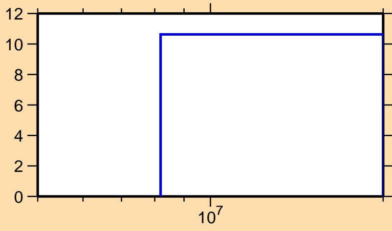
\Delta\sigma/\sigma vs. E for ^{137}\text{Te}(n,el.)
