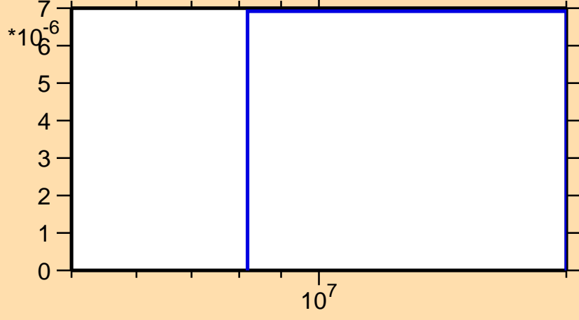
\sigma vs. E for ^{137}\text{Te}(n,d)
