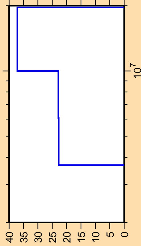
\Delta\sigma/\sigma vs. E for ^{138}\text{Te}(n,2n)
