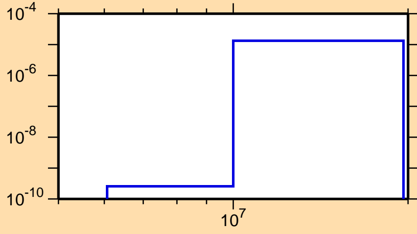
\sigma vs. E for ^{138}\text{Te}(n,n\alpha)
