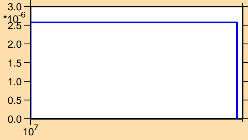
\sigma vs. E for ^{138}\text{Te}(n,p)
