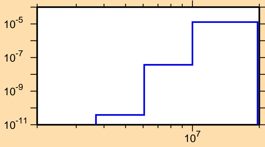
\sigma vs. E for ^{138}\text{Te}(n,\alpha)
