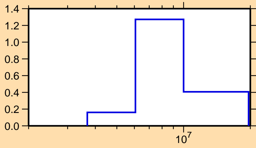
\sigma vs. E for ^{138}\text{Te}(n,2n)
