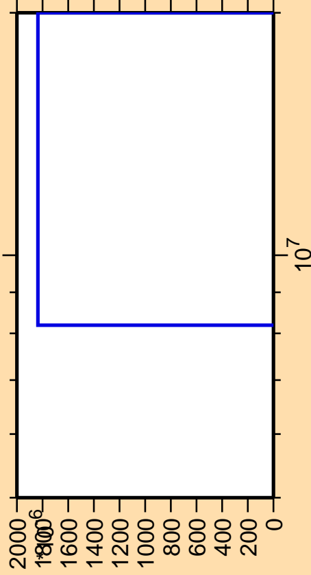
\Delta\sigma/\sigma vs. E for ^{138}\text{Te} (mt 11)
