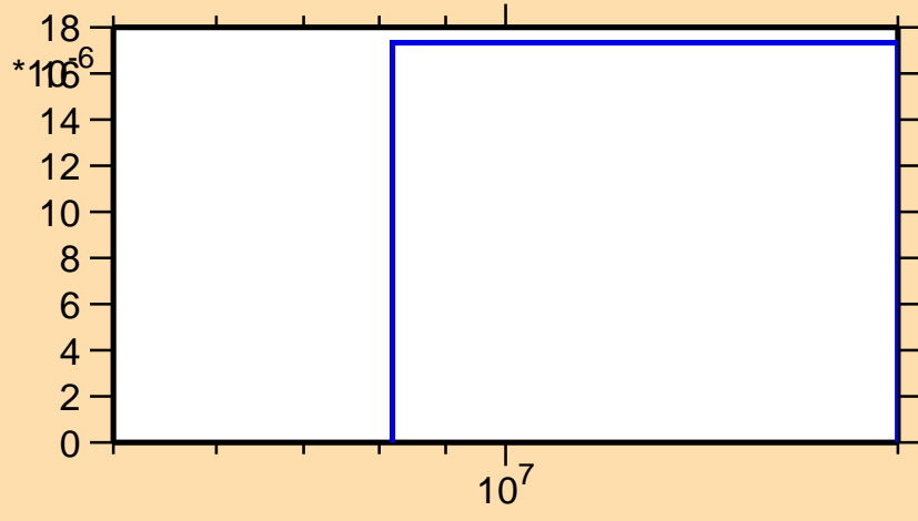
\sigma vs. E for ^{138}\text{Te}(n,t)
