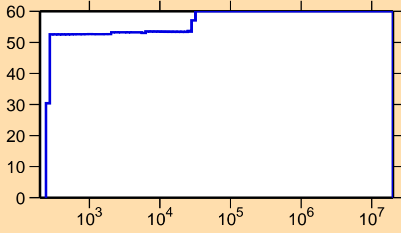
\Delta\sigma/\sigma vs. E for ^{215}\text{Th}(n,\gamma)
