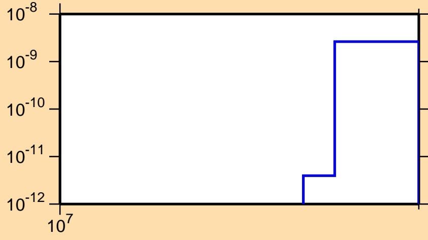
\sigma vs. E for ^{215}\text{Th}(n,nt)
