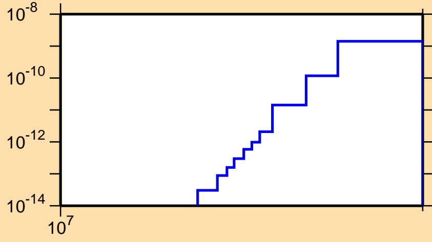
\sigma vs. E for ^{215}\text{Th}(\text{mt } 34)
