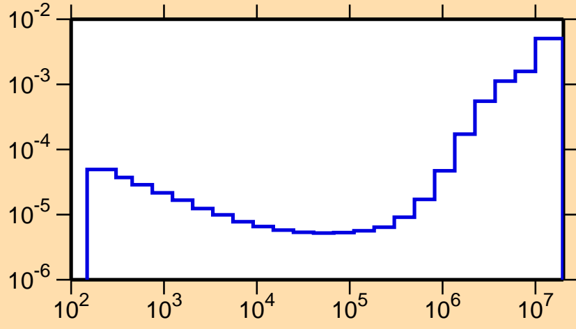
\sigma vs. E for ^{215}\text{Th}(n,p\alpha)
