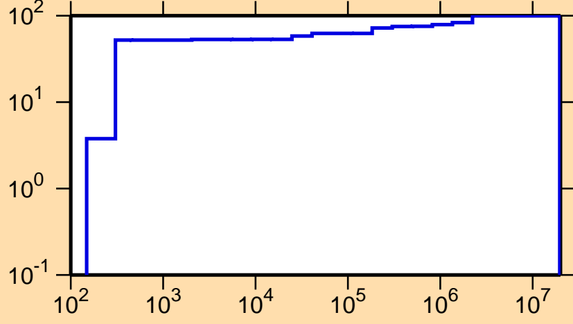
\Delta\sigma/\sigma vs. E for ^{215}\text{Th}(n,\gamma)
