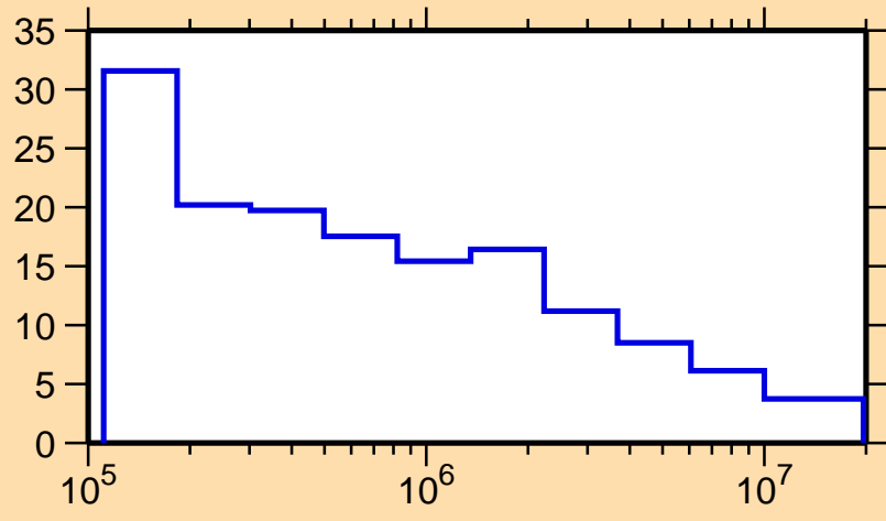
\Delta\sigma/\sigma vs. E for ^{215}\text{Th}(n,\text{nonel.})
