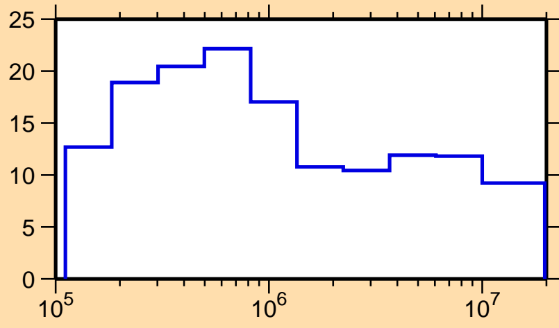
\Delta\sigma/\sigma vs. E for ^{215}\text{Th}(n,\text{el.})
